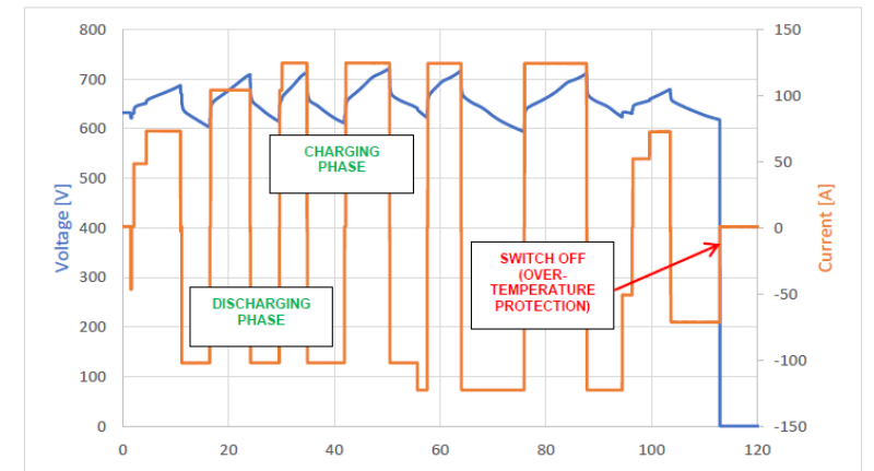
Over-temperature protection test
