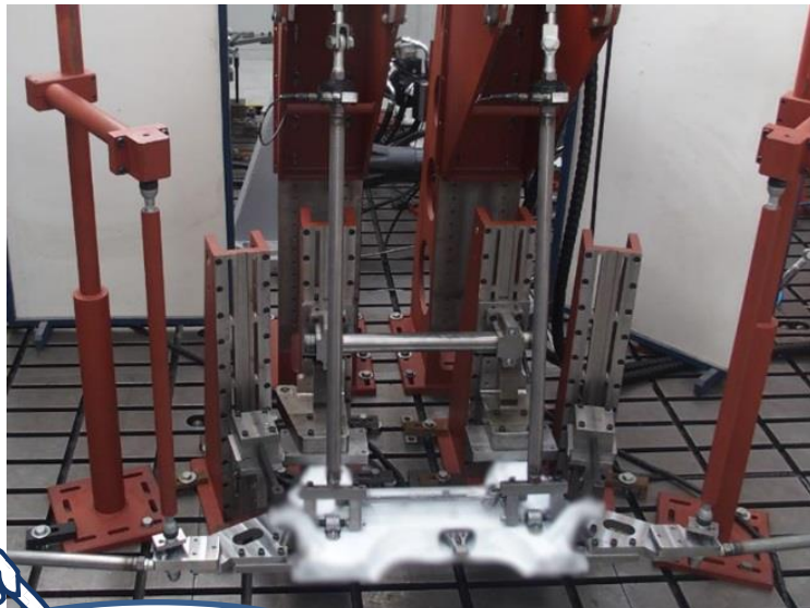
MTS and INOVA multiaxial test stands
