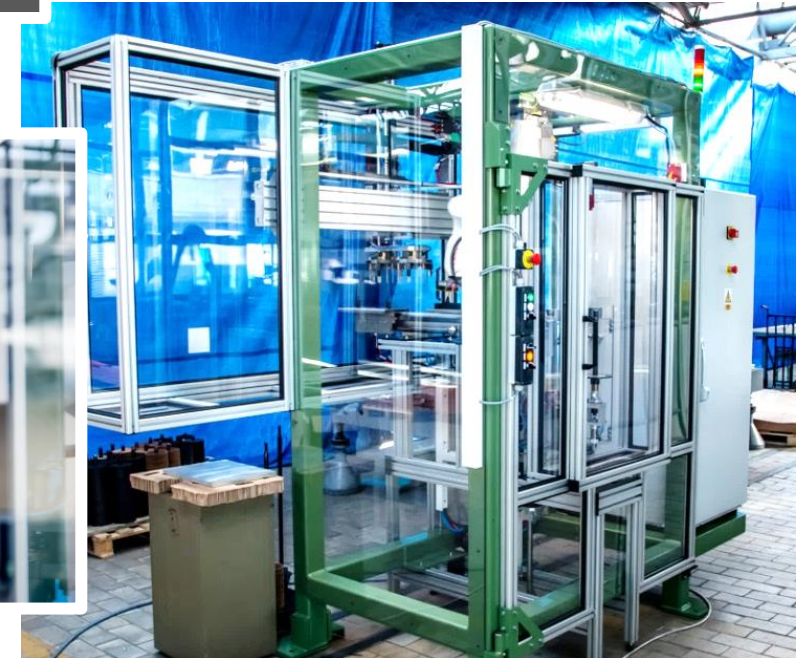
Example of concept, design and manufacturing of automated production line socket
