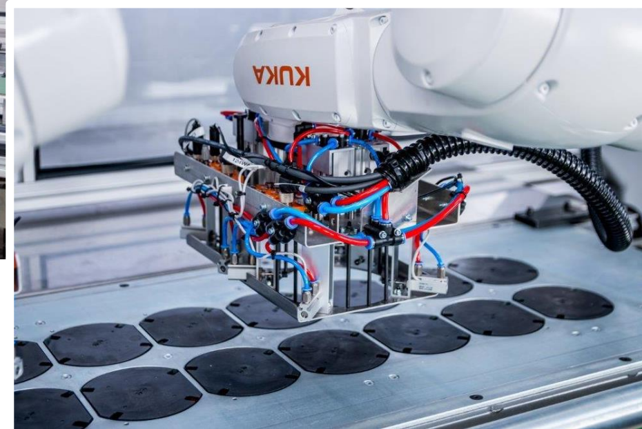
Example of special machine designed for automated production line socket
