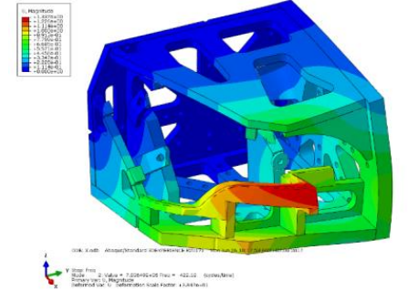
Natural frequency of holder
